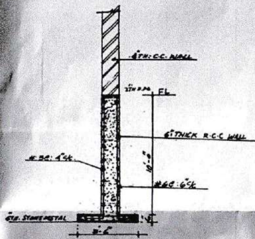
DETAIL OF 6TH WALL
